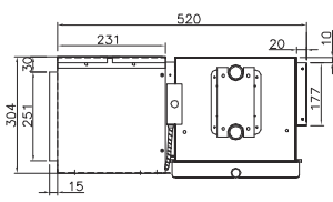
With back return air plenum (TCR1400)
