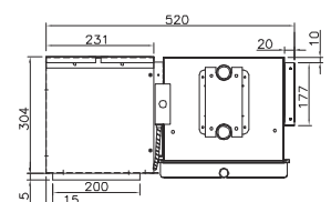
With bottom return air plenum (TCR1400)
