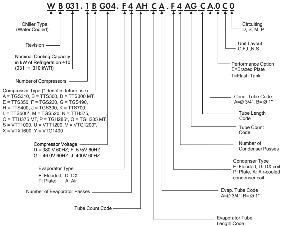
Model nomenclature for the Smardt T W -Class WB series chiller.
