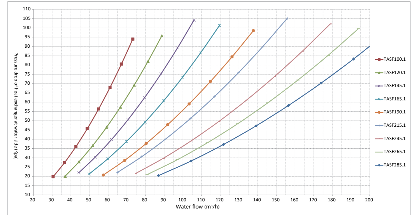
Water Pressure Drop Curve-Single Compressor(60Hz)
